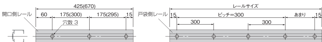
図4. AFD-1560TB-AFD-1360TB-HR-156TB-HR-136TB-SD-1160TB AFD-1560-AFD-1360-HR-156-HR-136-SD-1160
