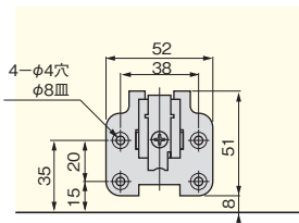
RLK-38座金
